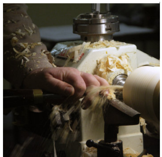
2 Forming the chuck recess
